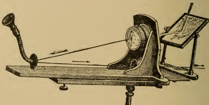
Fig. 45. BELL'S RADIOPHONE.
